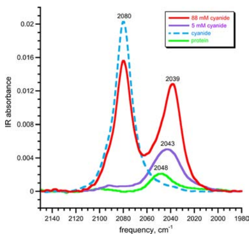
Figure 10. FTIR spectra of solutions of 1.1 mM Met121Ala iron(II)-azurin in 25 mM MOPS buffer at pH 10, with addition of 5 mM (purple) and 88 mM (red) cyanide. For comparison, the spectra of Met121Ala iron(II) azurin (green) and cyanide (blue dashed) are overlaid on the spectrum. The peak at 2080 \text{cm}^{-1} is due to free cyanide. The peak at 2043 \text{cm}^{-1} at low [\text{CN}^-] fits to the sum of two Lorentzian peaks (Figure S9, Supporting Information), consistent with a superposition of the residual protein peak at 2048 \text{cm}^{-1} and the C–N stretching band of the cyanide adduct at 2039 \text{cm}^{-1} .
