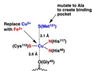
Figure 1. Metal site of the blue copper protein azurin, indicating changes intended to create an unsaturated iron site.
