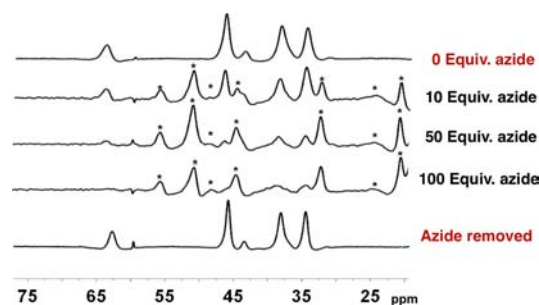
Figure 9. Portions of the {}^1\text{H} NMR spectra of iron(II)-substituted Met121Ala azurin (1.2 mM) with addition of \text{NaN}_3 . After the sequential additions, the azide was removed to generate the bottom spectrum.
