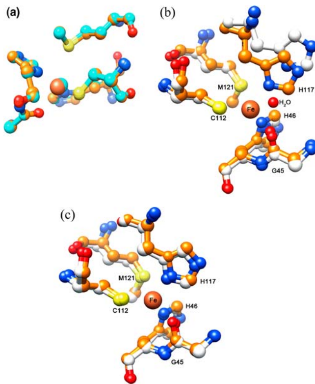
Figure 7. Metal site in the X-ray crystal structure of wild-type iron azurin. (a) Overlay of iron(II) (orange) and copper(II) (blue) azurins. (b) Overlay of chain B of iron(II) azurin (orange) with chain A of apo-azurin (white). The water molecule in apo-azurin is indicated. (c) Overlay of chain B of iron(II) azurin with chain B of apo-azurin.
