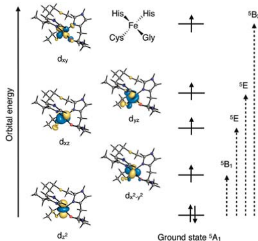
Figure 8. Metal d -based molecular orbitals for the wild-type iron(II)-azurin from a CASSCF calculation. The right side of the figure shows single excitations that lead to spin–orbit coupling, analyzed under approximate D_{2d} symmetry.
