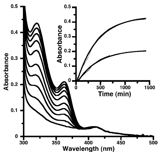
Figure 3. Growth of bands at 322 and 364 nm after the addition of 1 equiv of Fe^{2+} to wild type apo-azurin (0.18 mM). (Inset) Time course of the absorbance maxima of the two bands. The solid lines are exponential fits to the absorbances.
