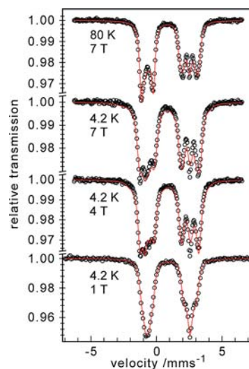
Figure 6. Magnetic Mössbauer spectra recorded at 4.2 and 80 K with fields of 1, 4, and 7 T applied perpendicular to the \gamma -rays. The red line is a spin Hamiltonian simulation for S = 2 with D = 14.3 \text{cm}^{-1} , E/D = -0.37 (corresponds to D = -15.1 \text{cm}^{-1} and E/D = 0.3 in the usual convention 0 \leq E/D \leq 1/3 , obtained by rotations with Euler angles \alpha = 90^\circ , \beta = 90^\circ ), A/g_N\beta_N = (-4.9, -5.4, -60.7) T, \Delta E_Q = -3.19 mm/s, \eta = 0.7 (efg rotated by \alpha = 19^\circ , \beta = 12^\circ ), \delta = 0.93 mm/s.
