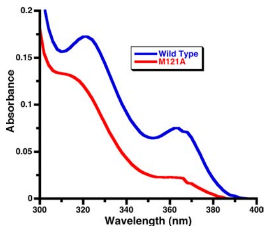
Figure 4. UV-vis spectra of iron(II) azurins (73 \mu M). (Top) Wild type. (Bottom) Met121Ala variant.
