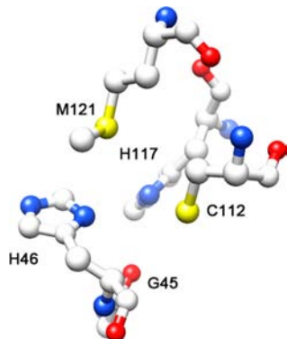
Figure 2. Unoccupied metal site in the X-ray crystal structure of apo-azurin (PDB 1E65). 26
